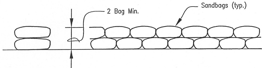
TYPICAL SECTION
